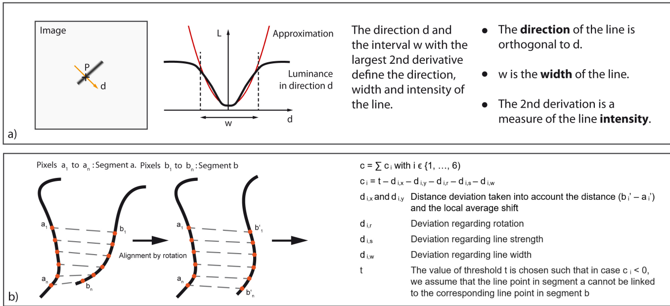
Fig. 3. a) Determining points of center lines using local approximations of the luminance by bivariate quadratic functions. b) Calculating the closeness c of two line segments.
